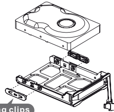
Locking clips
