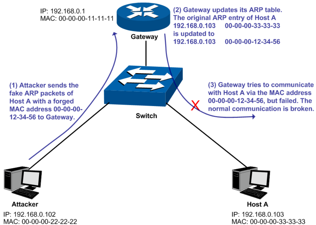
Figure 13-11 ARP Attack – Cheating Gateway
