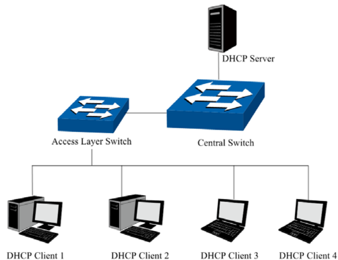
Figure 13-6 Network diagram for DHCP-snooping implementation
