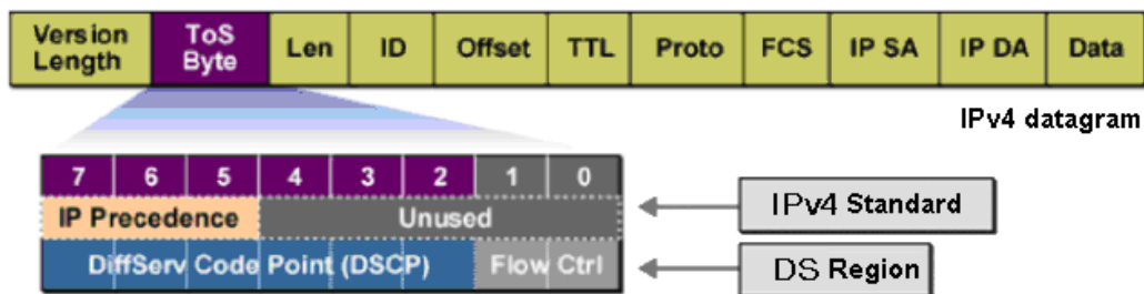
Figure 10-3 IP datagram
