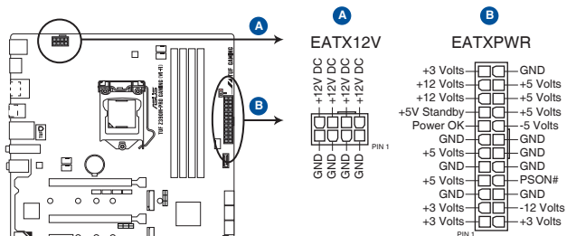
TUF Z390M-PRO GAMING (WI-FI) EATX power connectors
